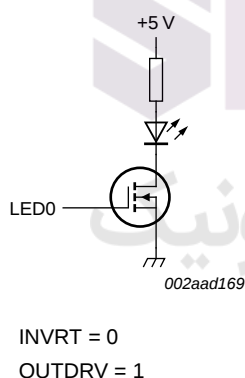
Fig 13. External N-type driver
