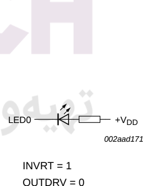
Fig 15. Direct LED connection
