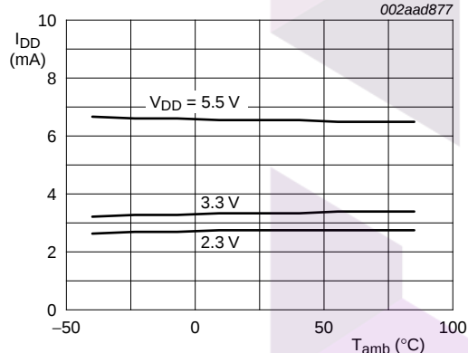
Fig 28. I_{DD} typical values with OSC on and f_{SCL} = 1\text{ MHz} versus temperature
