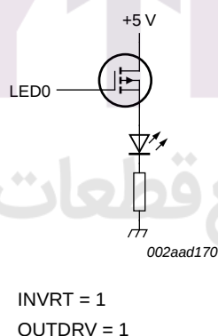
Fig 14. External P-type driver
